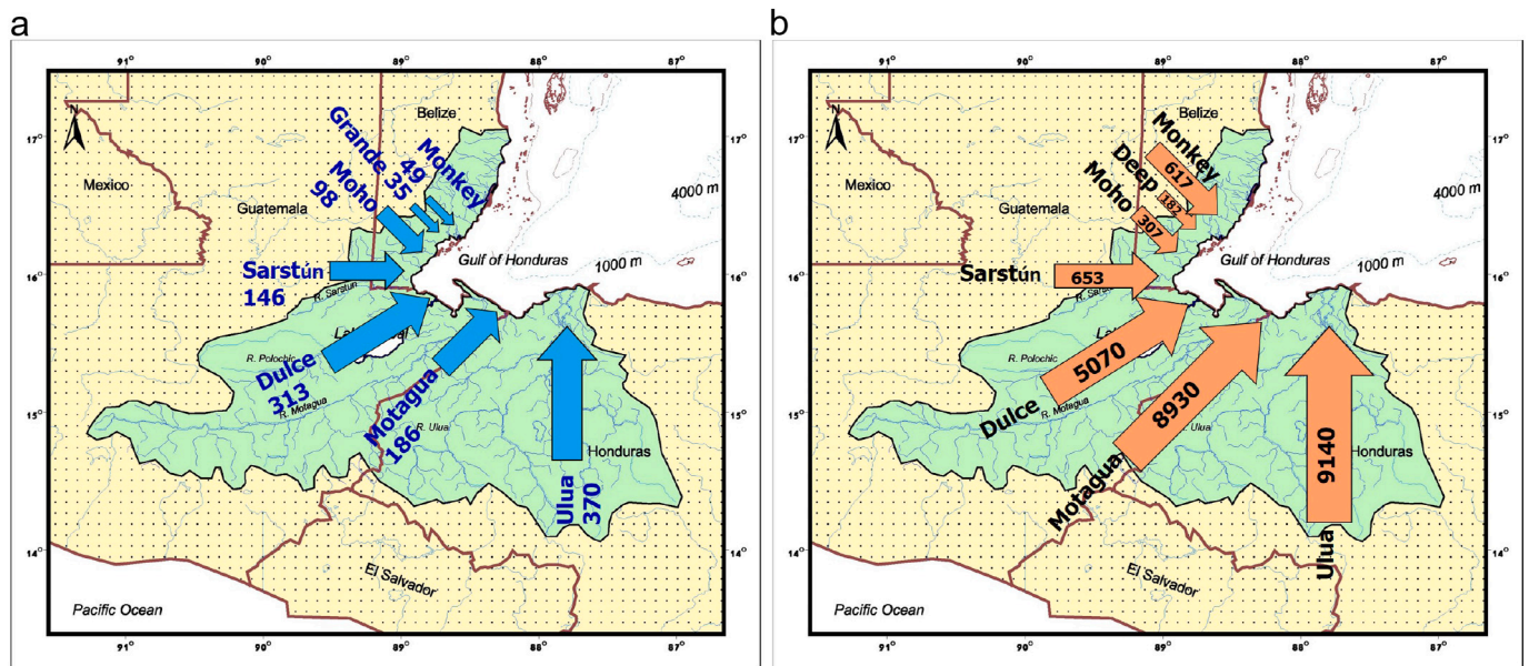
Fig. 2. (a) Modeled mean annual water discharge ( \text{m}^3/\text{s} ) and (b) modeled annual sediment discharge ( 10^3 \text{ t yr}^{-1} ) into the southern Belize Barrier Reef lagoon, Bahía de Amatique, and the Gulf of Honduras.
