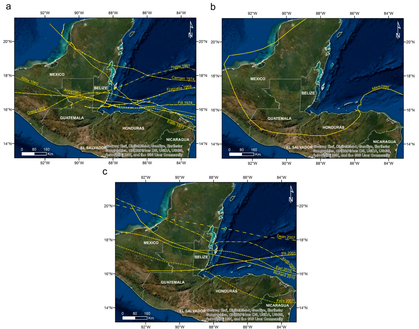
Fig. 3. Tracks of all hurricanes crossing and impacting the Gulf of Honduras (a) 1960–1979, (b) 1980–1999, and (c) 2000–2019.
